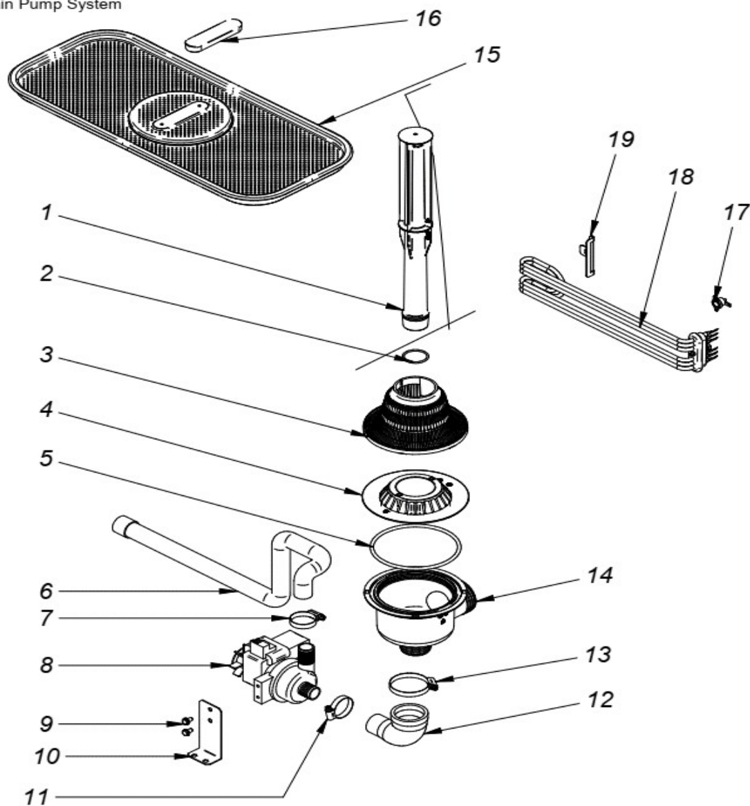
Drain Pump System
