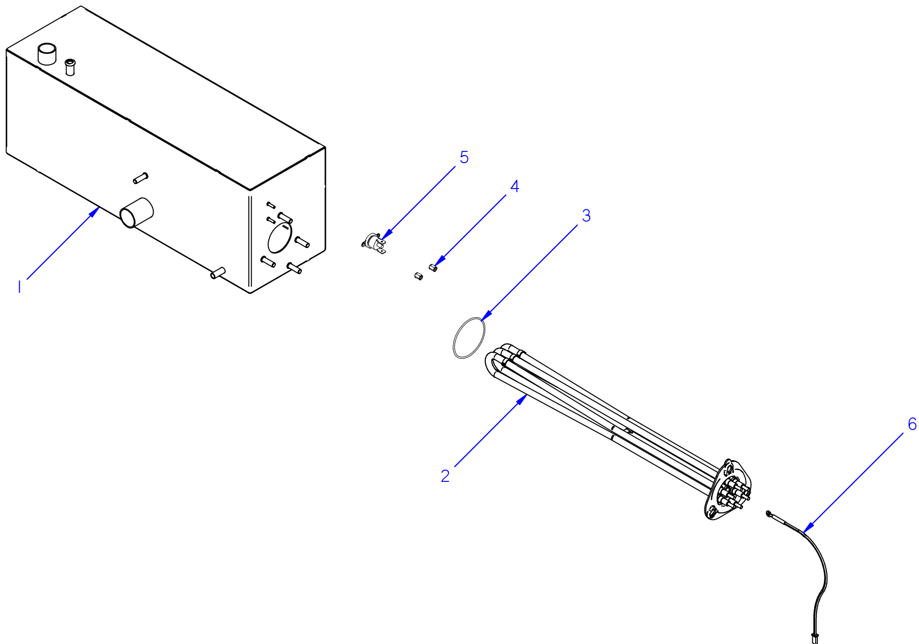
Calderín / Heater – GLB0071/FN / GLB0080N / GLB0082N
