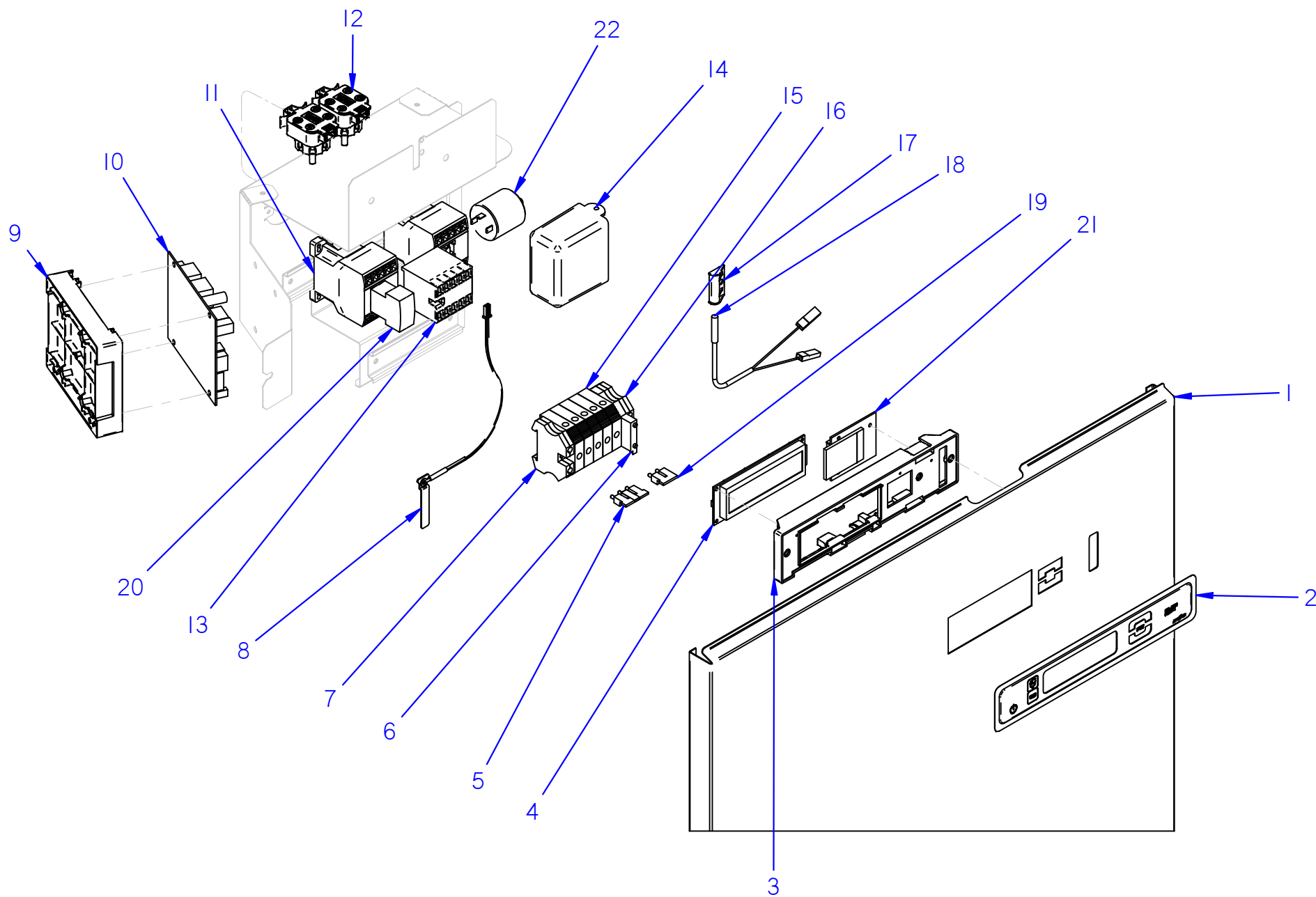
Portamandos / Control holder – GLB0080N
