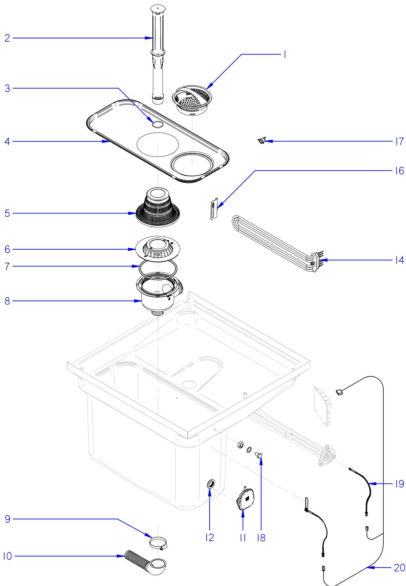
Componentes cuba / Tank parts – GLB0071/FN / GLB0082N
