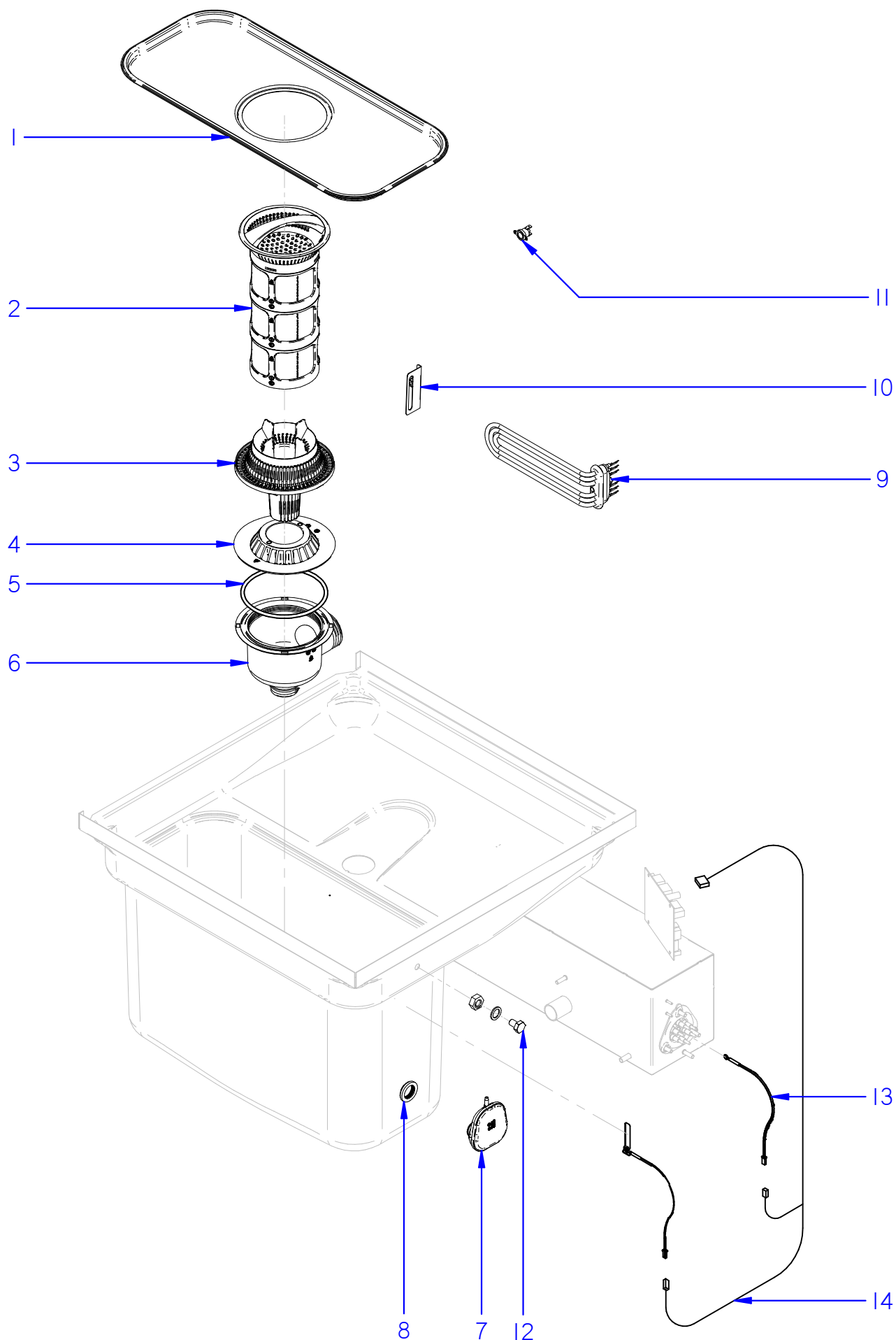
Componentes cuba / Tank parts – GLB0080N
