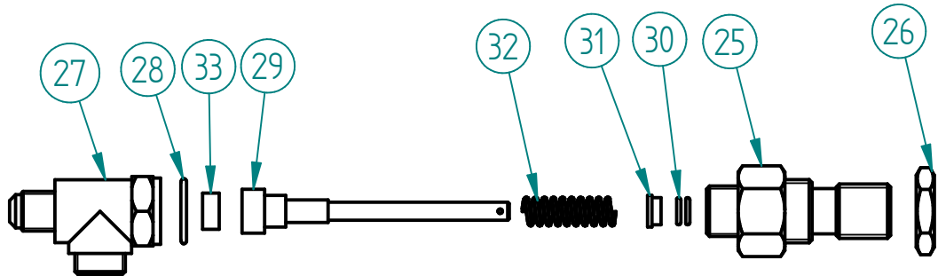
15 / 20 – 5.0.016.0350 – TORNEIRA ECC-07 G1/4-G1/8F 15 / 20 – TAP ECC-07
