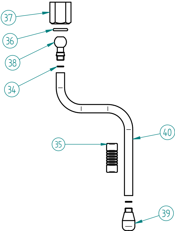
19 – 5.0.016.0320 – TUBO TORNEIRA VAPOR ATLANTIC (CONJ.) 19 – STEAM TAP TUBE ASS.
