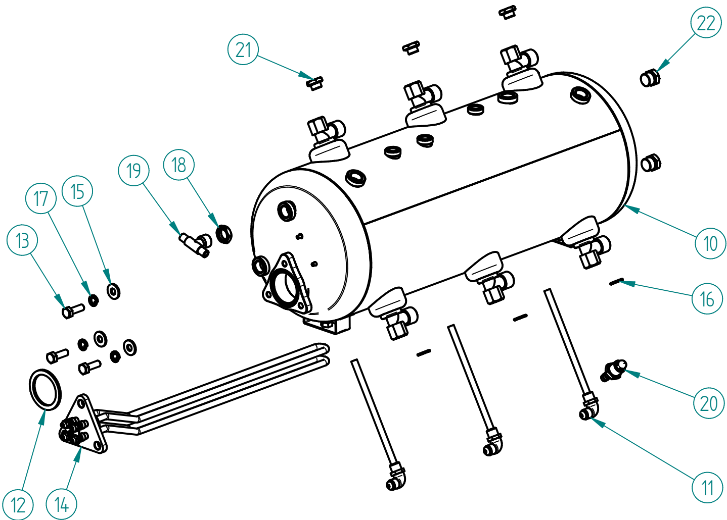
1 - 7.0.000.0516 - CALDEIRA 3GR 17 LT C/ ACESS. 1 - 3 GROUP 18 LT BOILER W/ ACESS.
