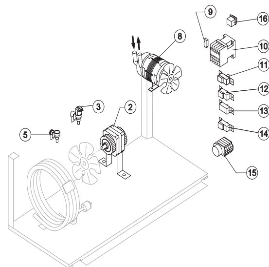
ELECTRIC PARTS
