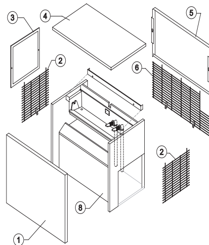
SHELL ASSY
