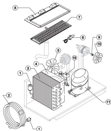
COOLING SYSTEM
