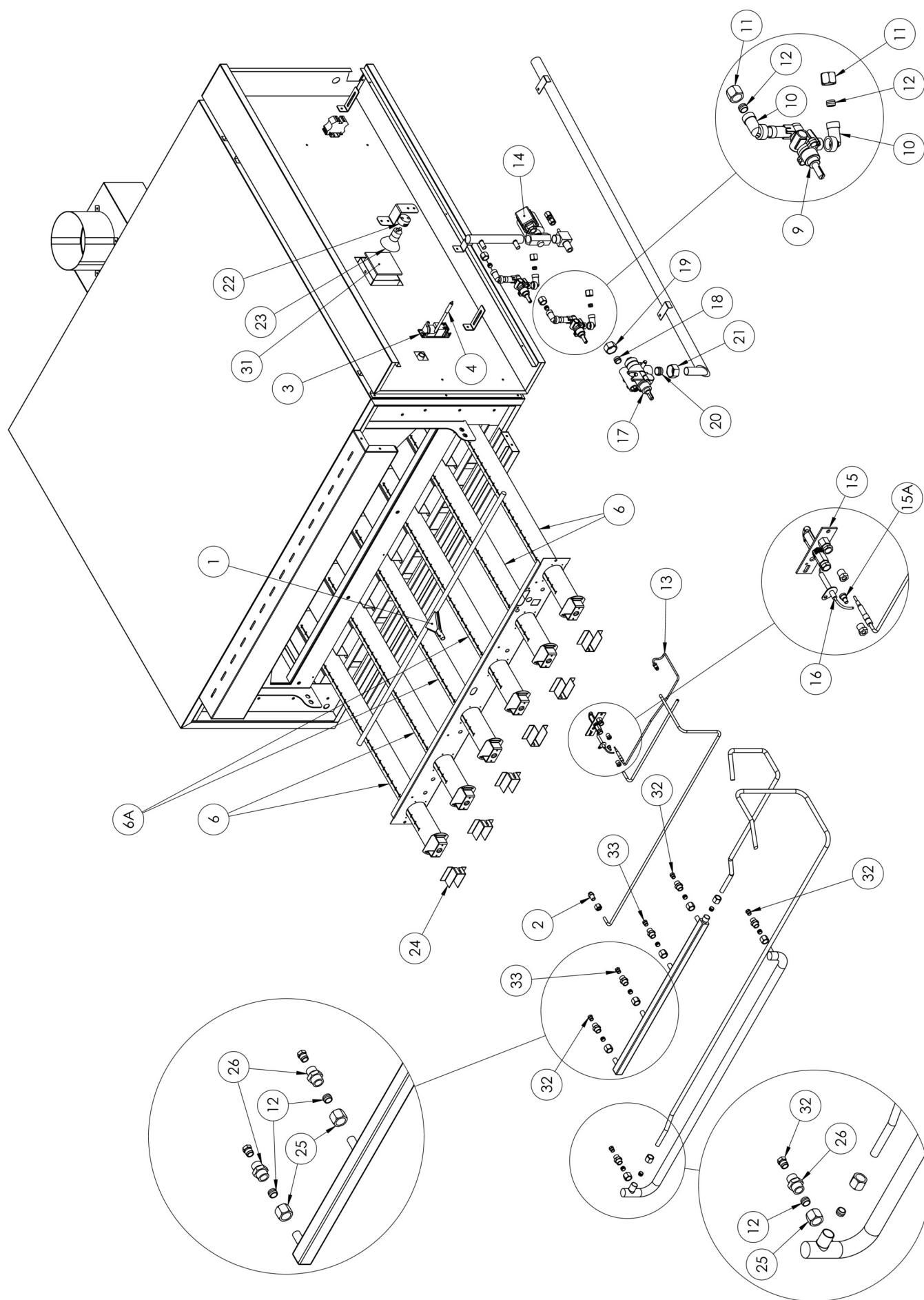
FIG.21 (exploded view mod G9)
