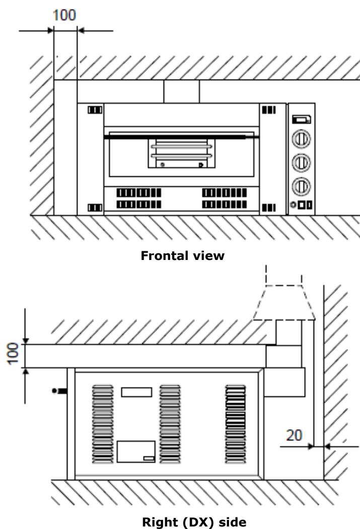
FIG.5 (Minimal measurements of positioning)
